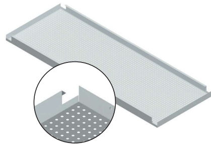
Painel CLIP-IN 3 FLEX 1200 x 300 mm
