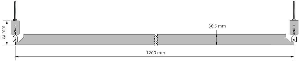
CLIP-IN 1 FLEX 1200 x 300 mm
