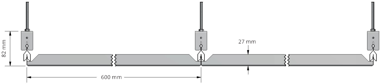
CLIP-IN 1 FLEX 600 x 600 mm
